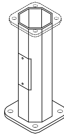
PEDESTAL ADAPTOR DETAIL
